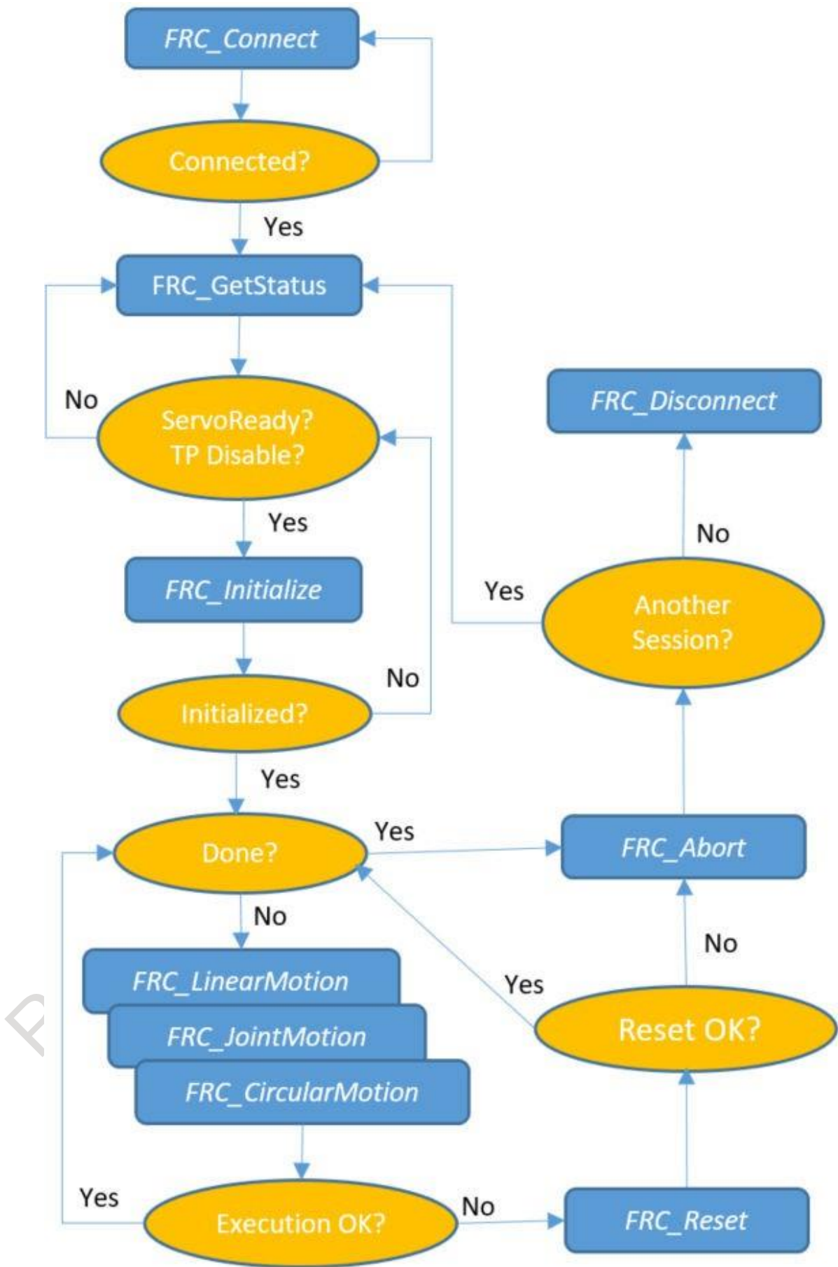
Figure 3.1 Remote Device Control Flow Chart
